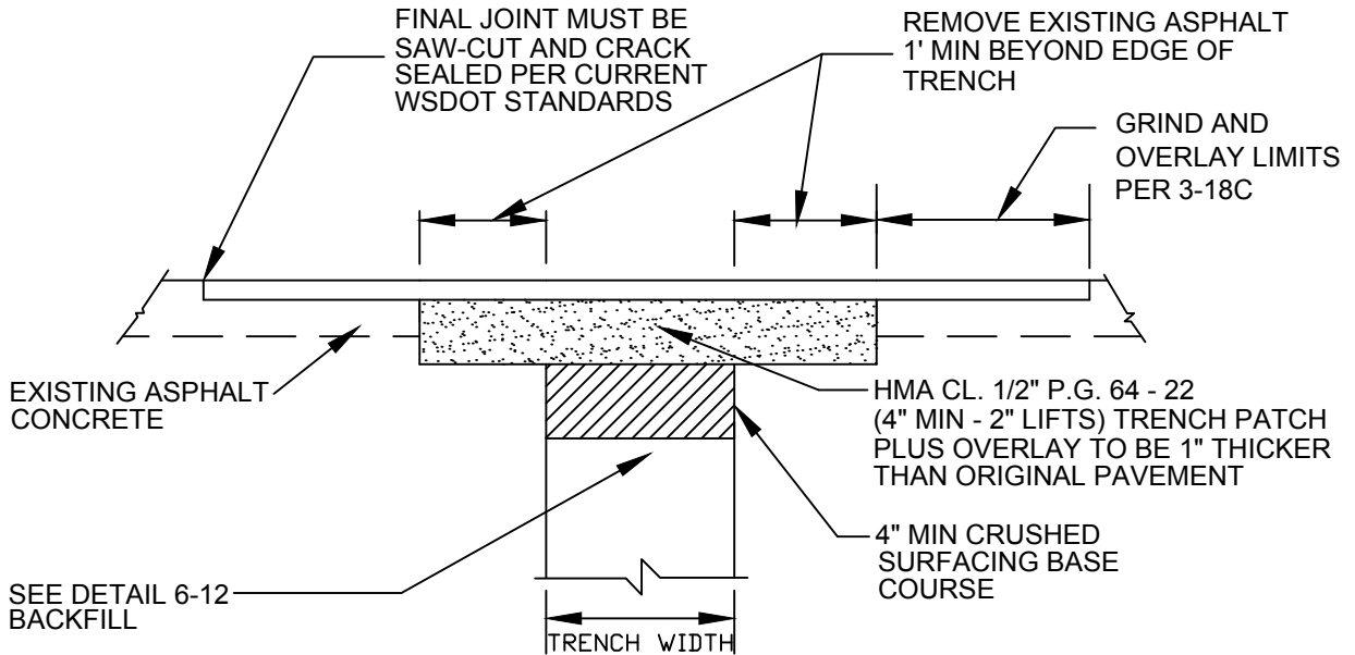
PAVEMENT PATCH
