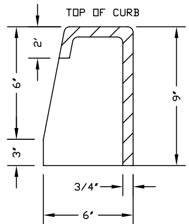
SECTION VIEW
