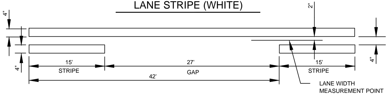
TWO WAY LEFT TURN STRIPE (YELLOW)
