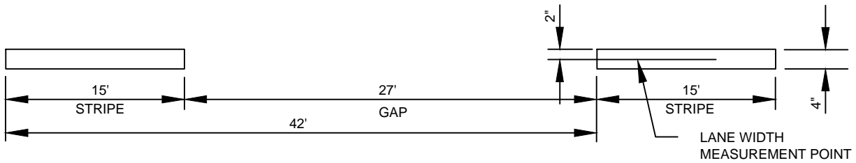
LANE STRIPE (WHITE)
