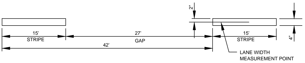
SKIP CENTER STRIPE (YELLOW)
