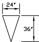
TOOTH DETAIL
