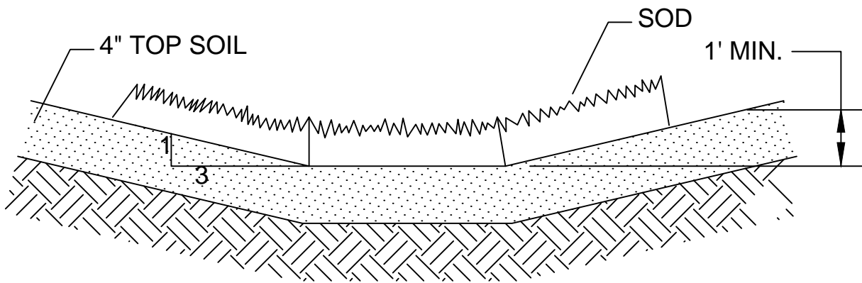
VEGETATED SWALE CROSS SECTION
