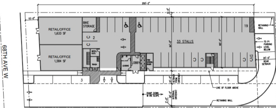
FIRST FLOOR PLAN / SITE PLAN
