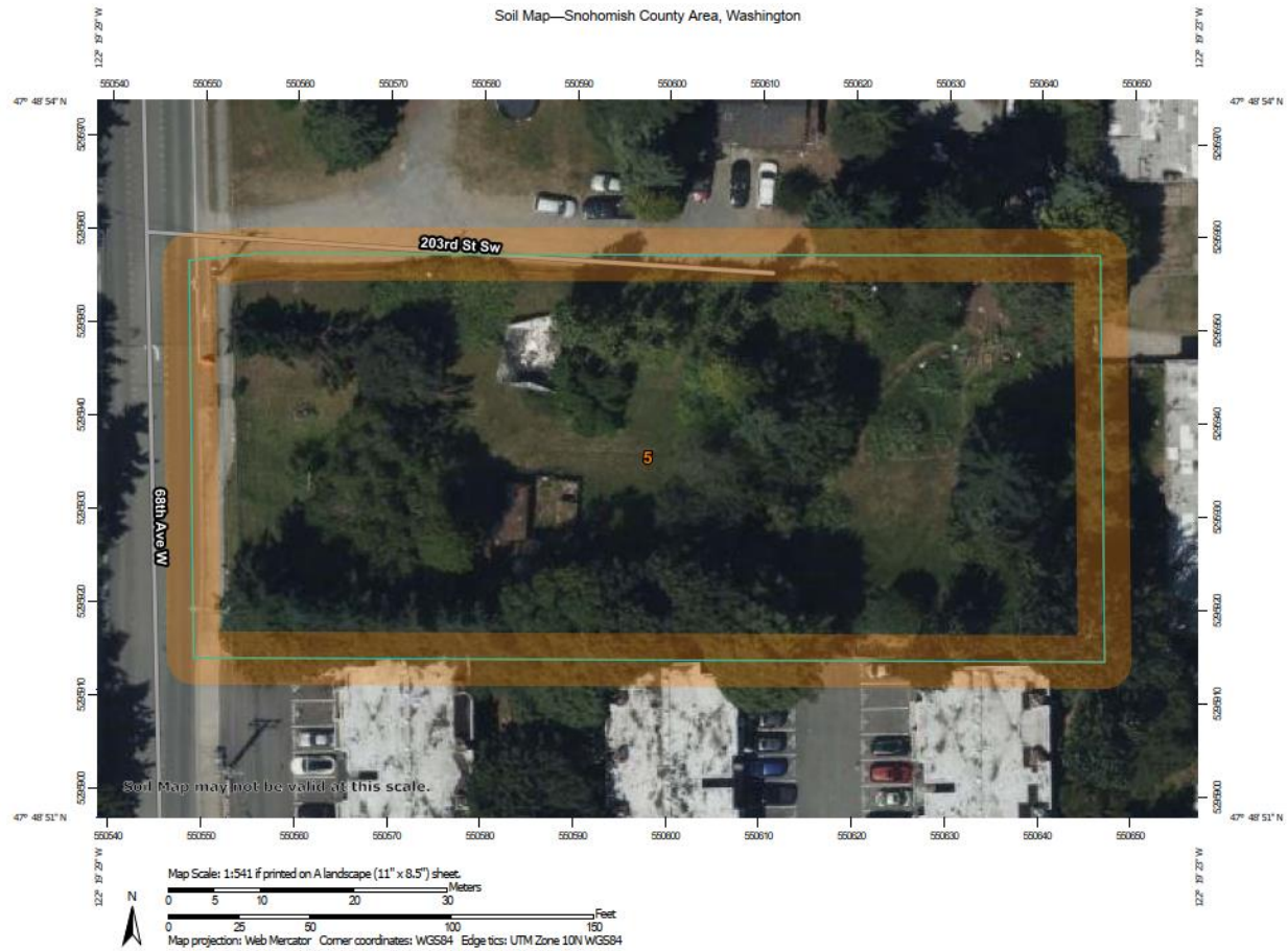
FIGURE 3 SOILS MAP
