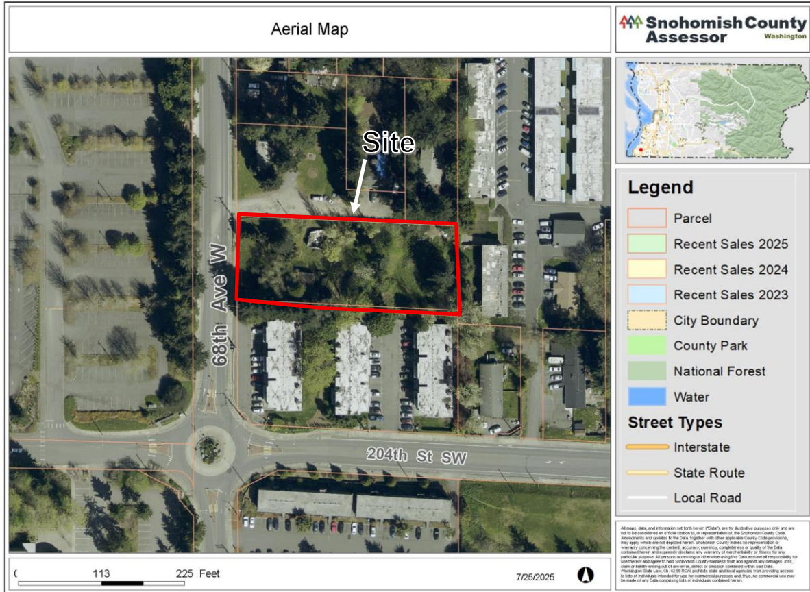
FIGURE 4 AERIAL MAP
