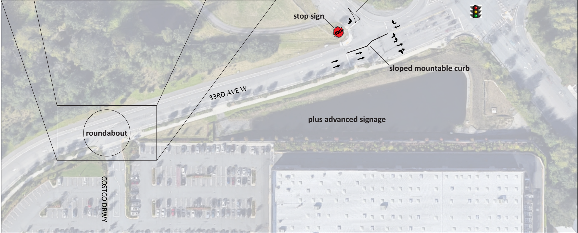
Figure 4: Alternative 1 Conceptual Improvements
