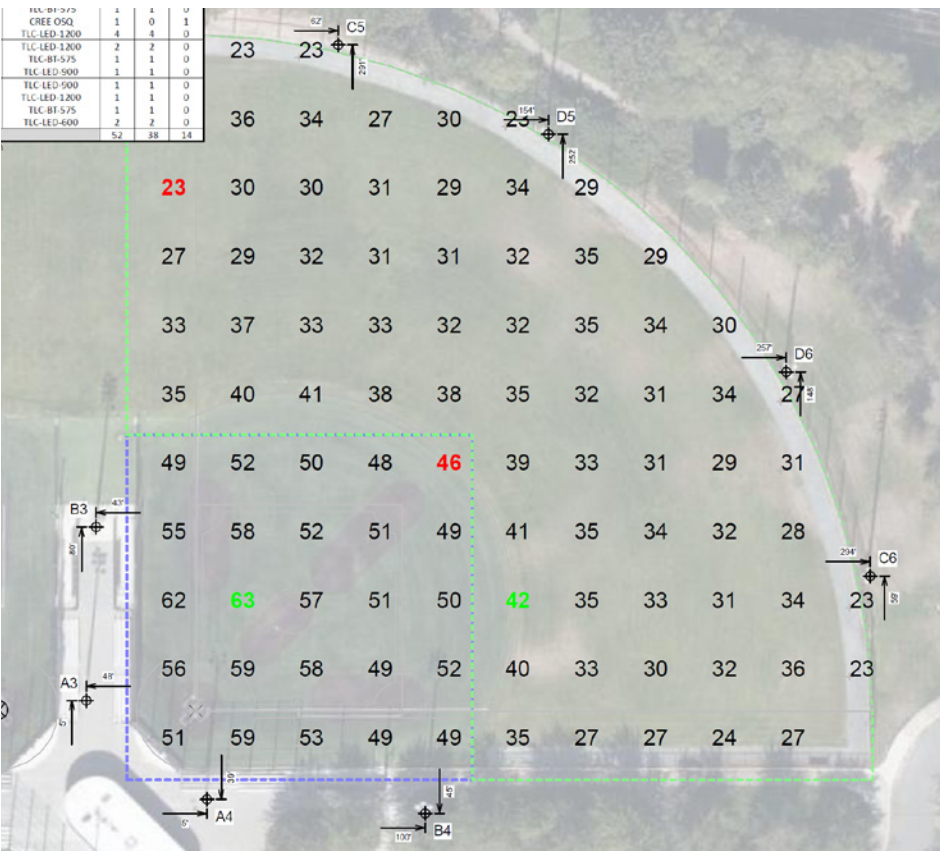
FIELD #2 Guaranteed Average Footcandle Performance: 30
