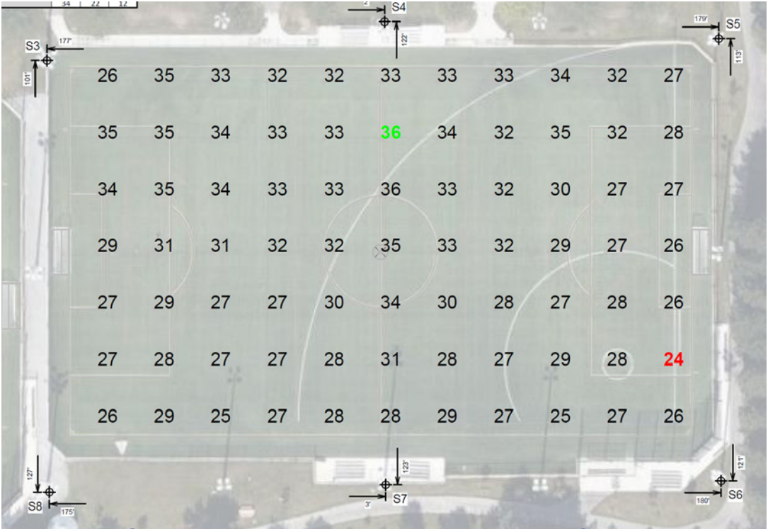
FIELD #1 Guaranteed Average Footcandle Performance: 30
