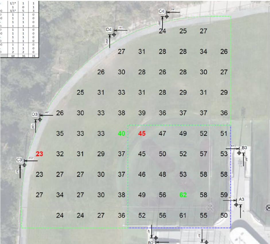
FIELD #1 Guaranteed Average Footcandle Performance: 30
