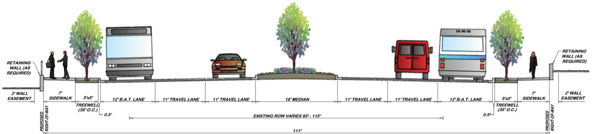
PROPOSED 196TH ST SW WITH 18' MEDIAN
