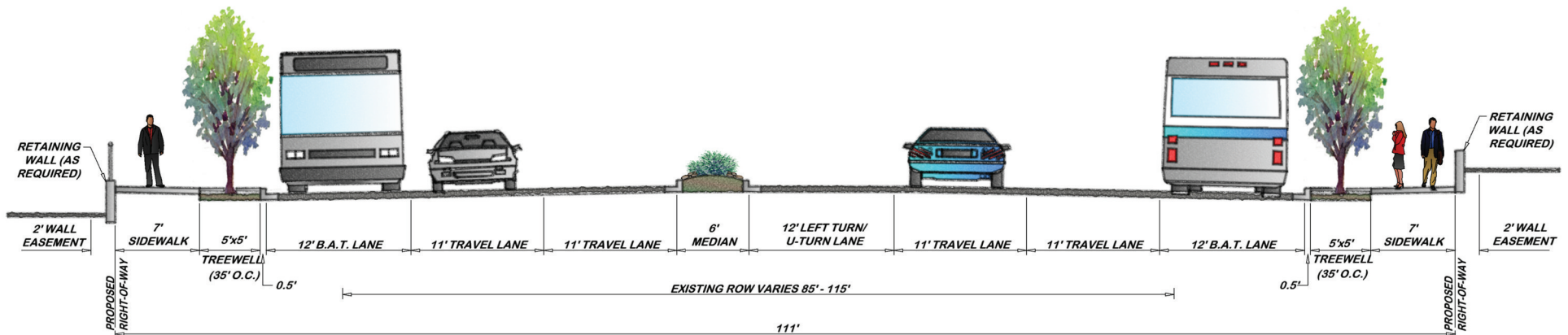
PROPOSED 196TH ST SW WITH LEFT TURN LANE AND 6' MEDIAN
