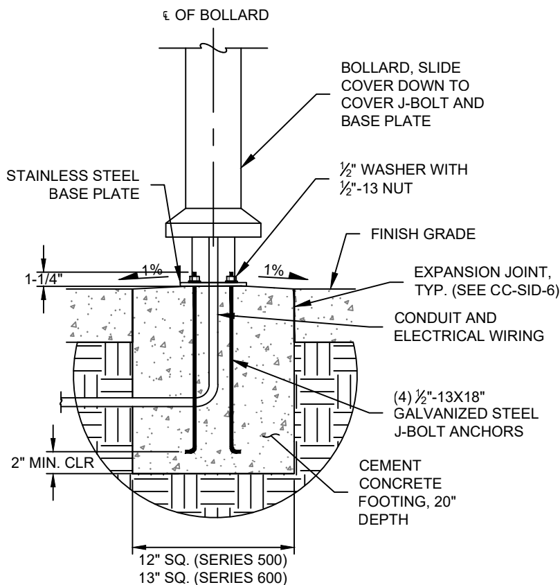
EMBED MOUNT
