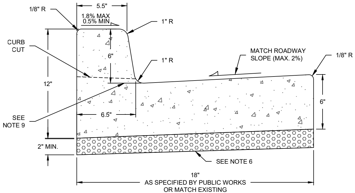
TYPICAL SECTION
