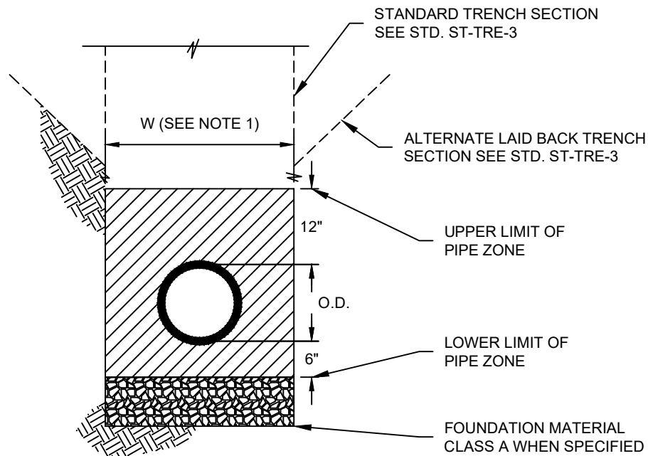
SECTION: PIPE BEDDING
