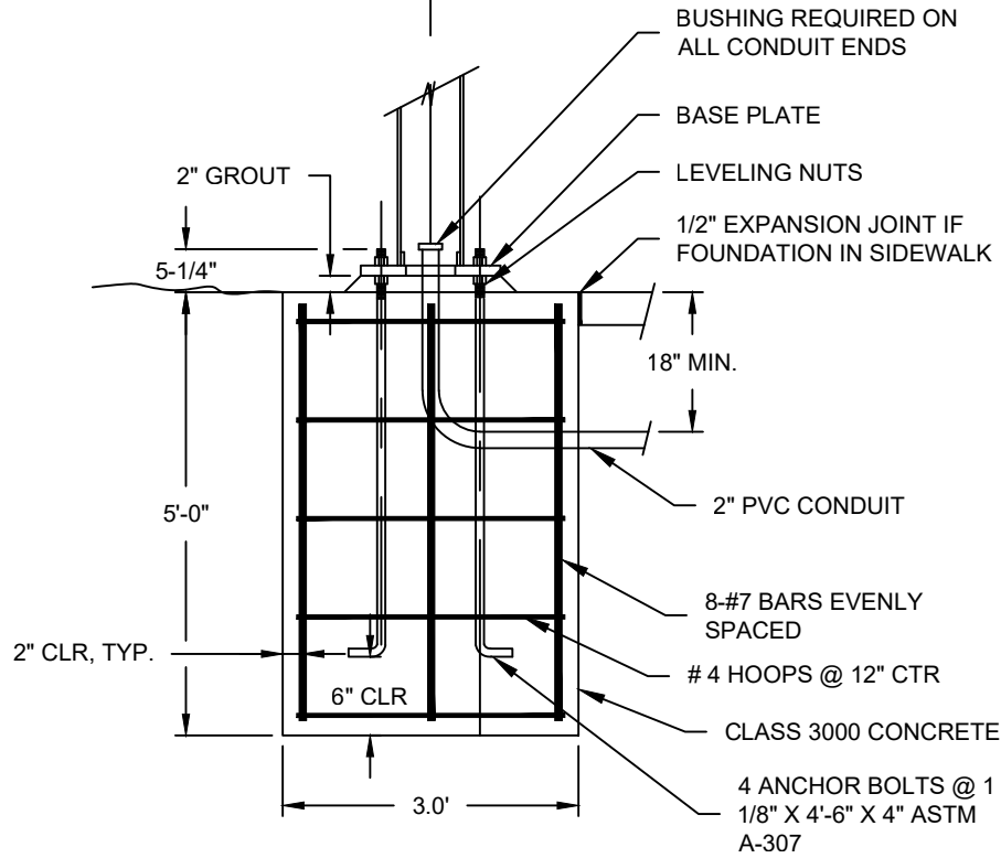
FOUNDATION SECTION
