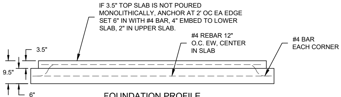
FOUNDATION PROFILE
