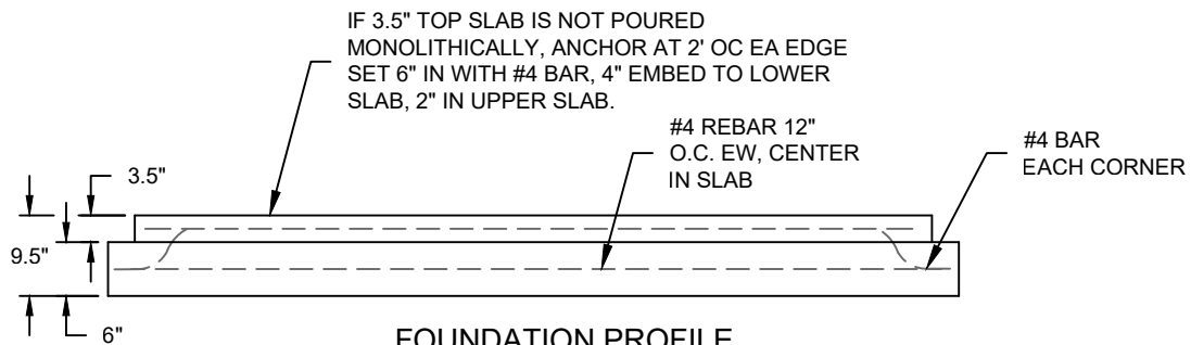
FOUNDATION PROFILE
