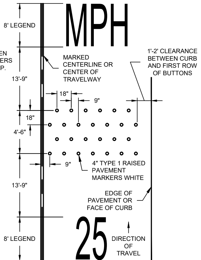
RUMBLE STRIP WITH 25 MPH LEGEND
