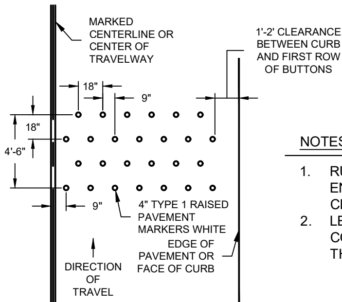
RUMBLE STRIP
