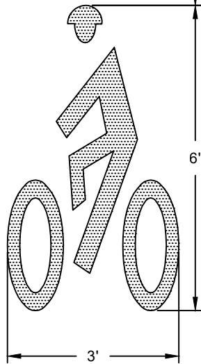
BIKE LANE SYMBOL DETAIL
