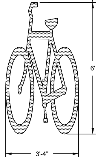
SHARED LANE SYMBOL DETAIL
