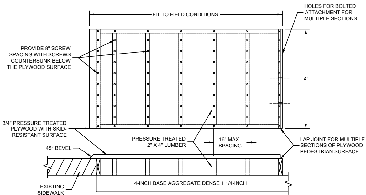
PLAN & PROFILE NTS
