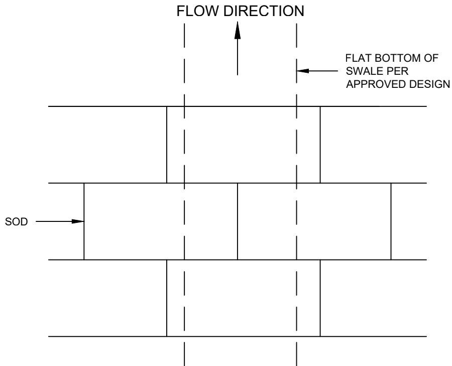
VEGETATED SWALE PLAN VIEW
